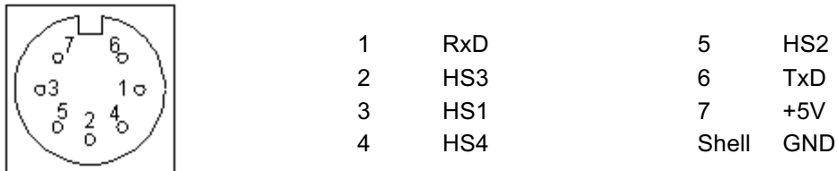
Figure 4: Pin assignment of handswitch socket; pin alignment according to DIN 45329
