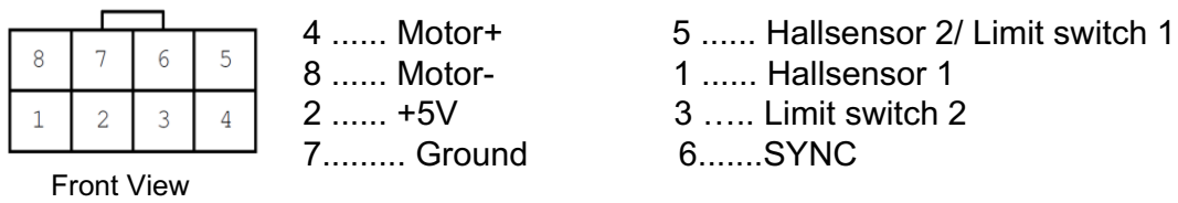
Figure 3: Pin assignment of motor socket
